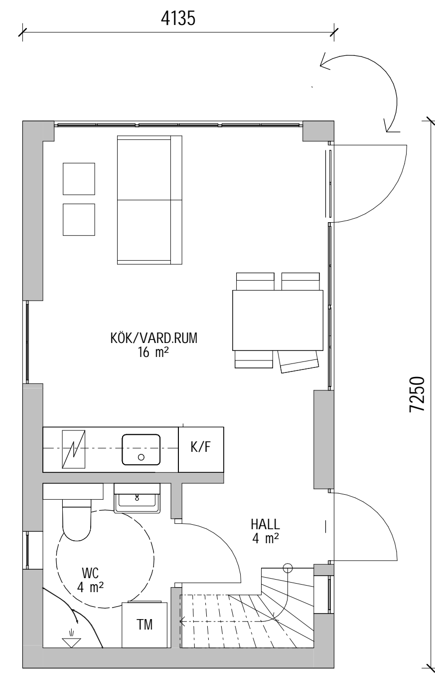
PLAN
